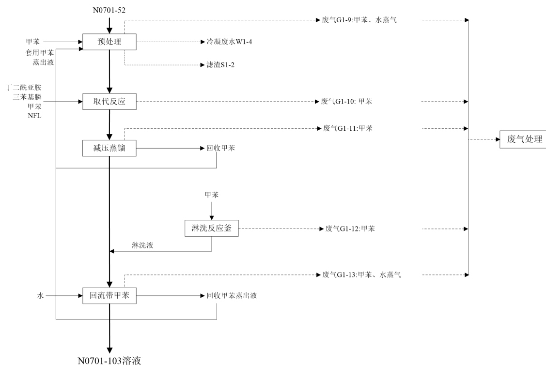
图3.3.2.3-2 N0701-108制备工段生产工艺流程图-1
