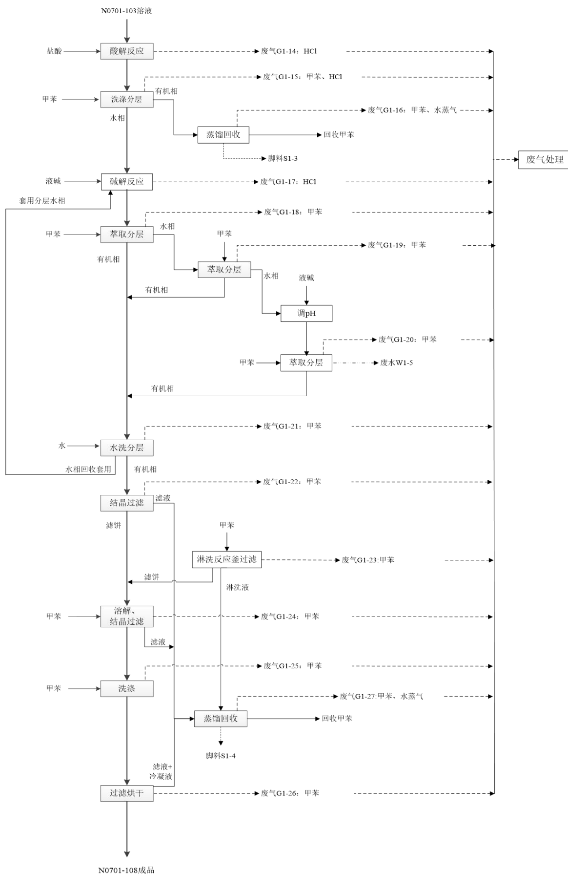
图3.3.2.3-3 N0701-108制备工段生产工艺流程图-2
